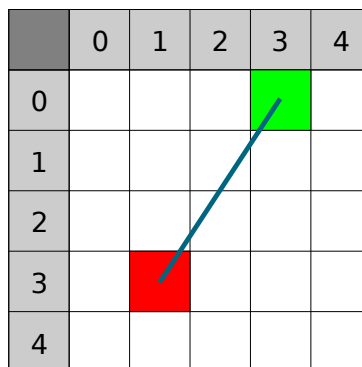
Figure 331: Example of Euclidean Distance
